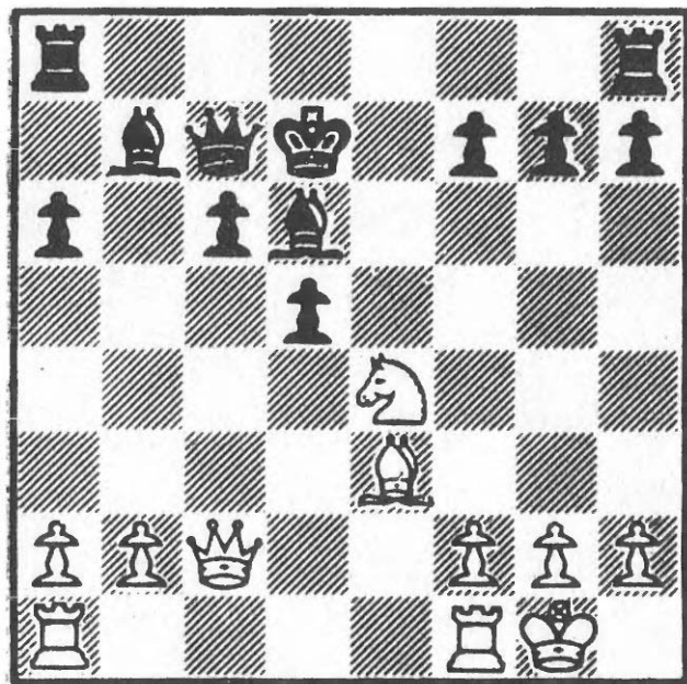
335 After 17...exd5
